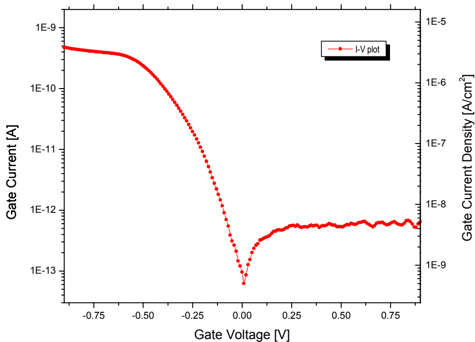
Fig. 3: I-V curve measured on a fully annealed sample grown at 800°C.
