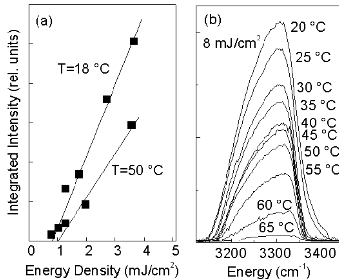
Fig. 2: Dependence of the stimulated emission of sample 1 on excitation intensity (a) and on sample temperature (b). Laser operation is obtained up to 65^\circ\text{C} .
