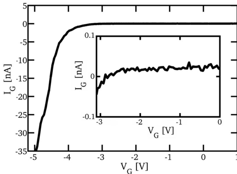
Fig. 2: I-V-characteristics of all gates connected in parallel to maximize possible leakage currents. Down to about -3 \text{ V} the leaking currents are below the measurement accuracy. The insert shows a zoom-in of the non-conducting range of the diode characteristics.
